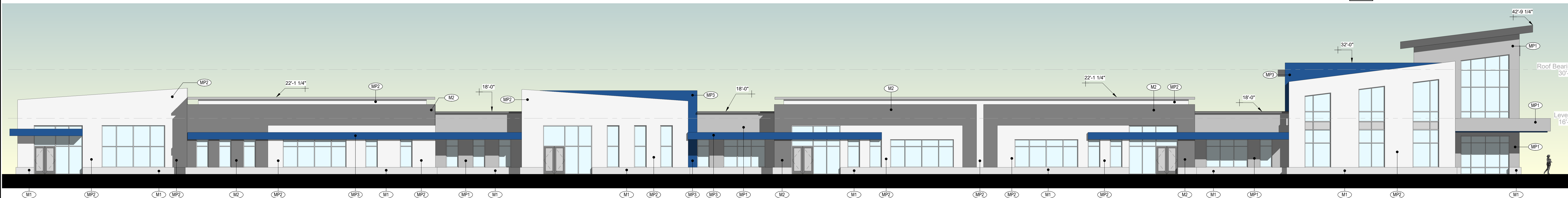
1 Elevation - 28th St. SD2.103 3/32\" = 1'-0"
