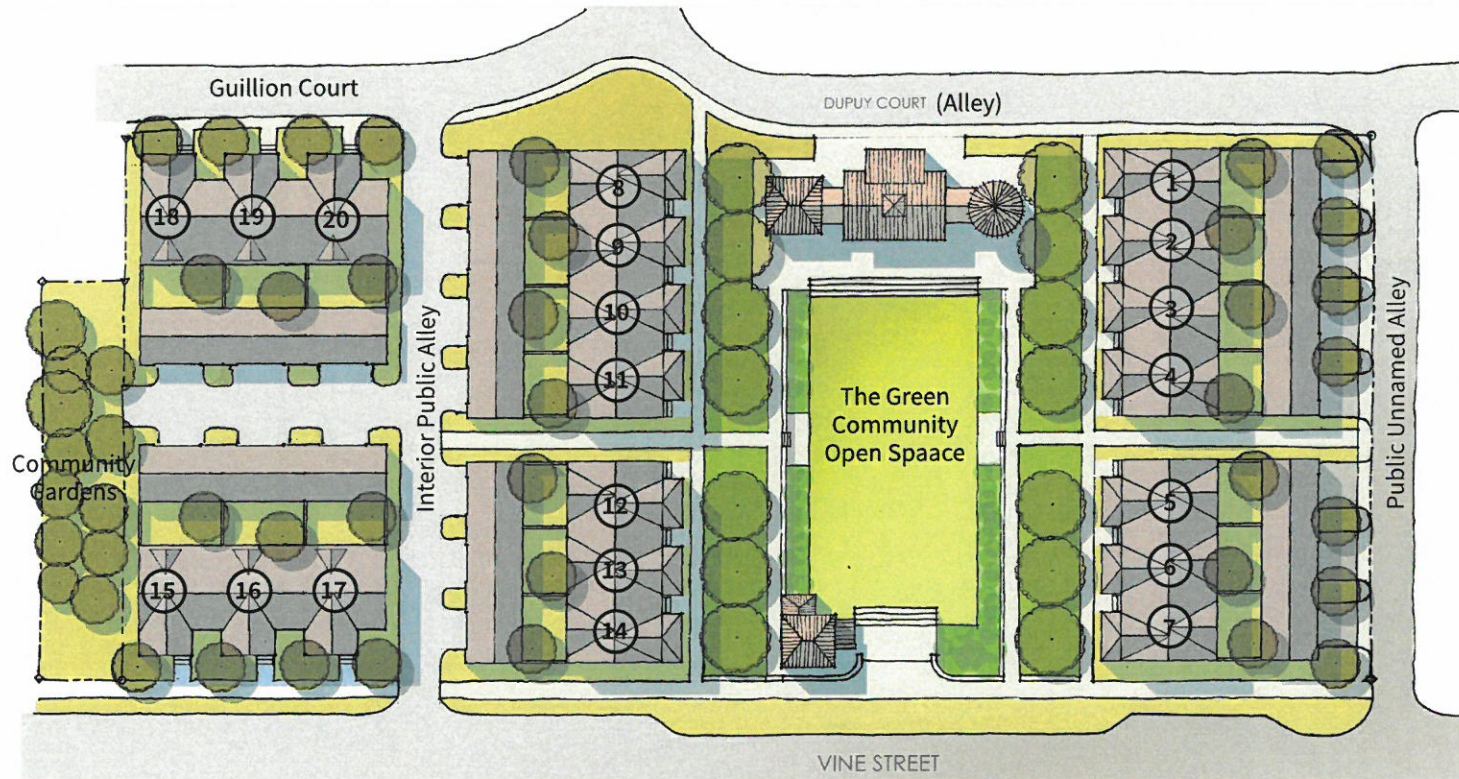
Site Plan Concept
