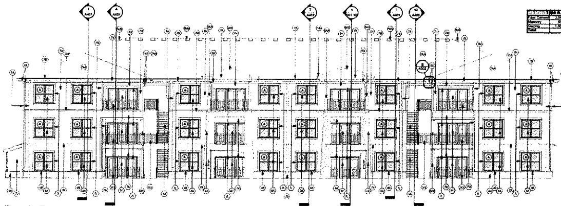
1 Elevation - Type A - Front A201 1/8" = 1'-0"
