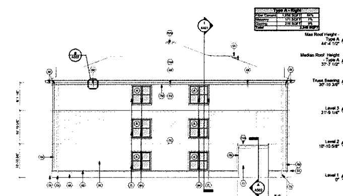
4 Elevation - Type A - Right A201 1/8" = 1'-0"
