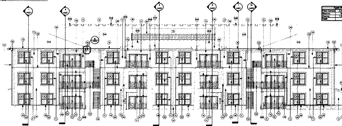
2 Elevation - Type A - Rear A201 1/8" = 1'-0"
