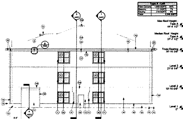
3 Elevation - Type A - Left A201 1/8" = 1'-0"
