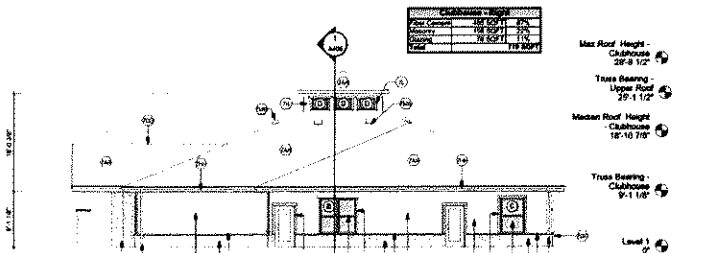
4 Elevation - Clubhouse - Right A211 1/8" = 1'-0"
