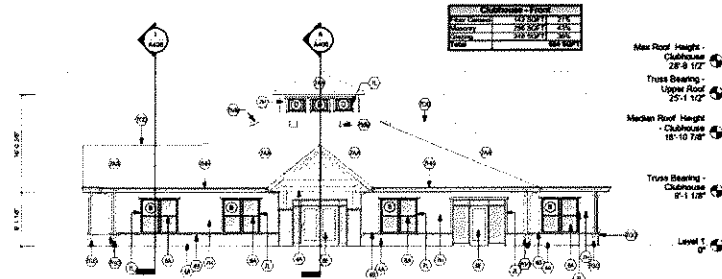
1 Elevation - Clubhouse - Front A211 1/8" = 1'-0"
