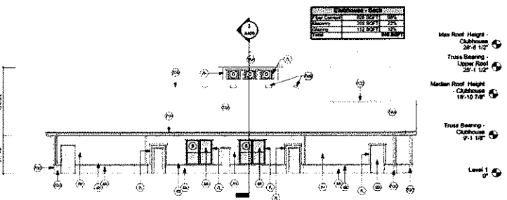
2 Elevation - Clubhouse - Rear A211 1/8" = 1'-0"
