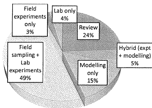
Fig. 7. Breakdown of methodological approaches.
