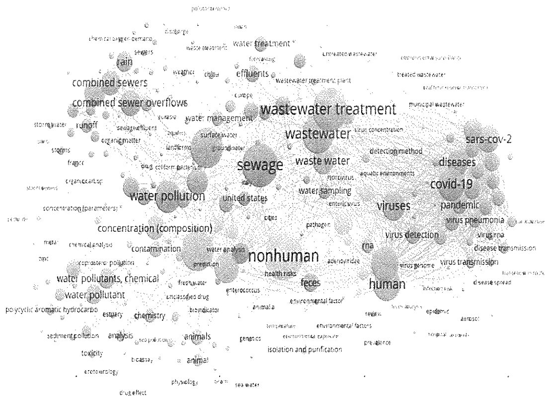
Fig. 2. Co-occurrence of keywords network.
