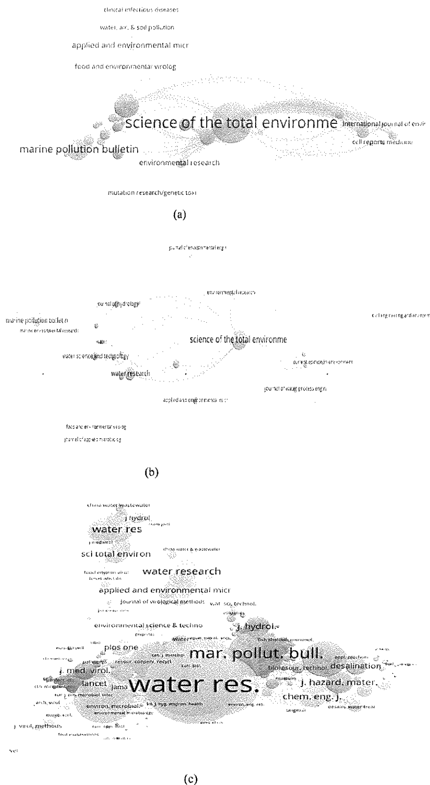
Fig. 3. (a) Network of journal contribution. (b) Publication outlets by documents (c) Publication outlet based on co-citations.
