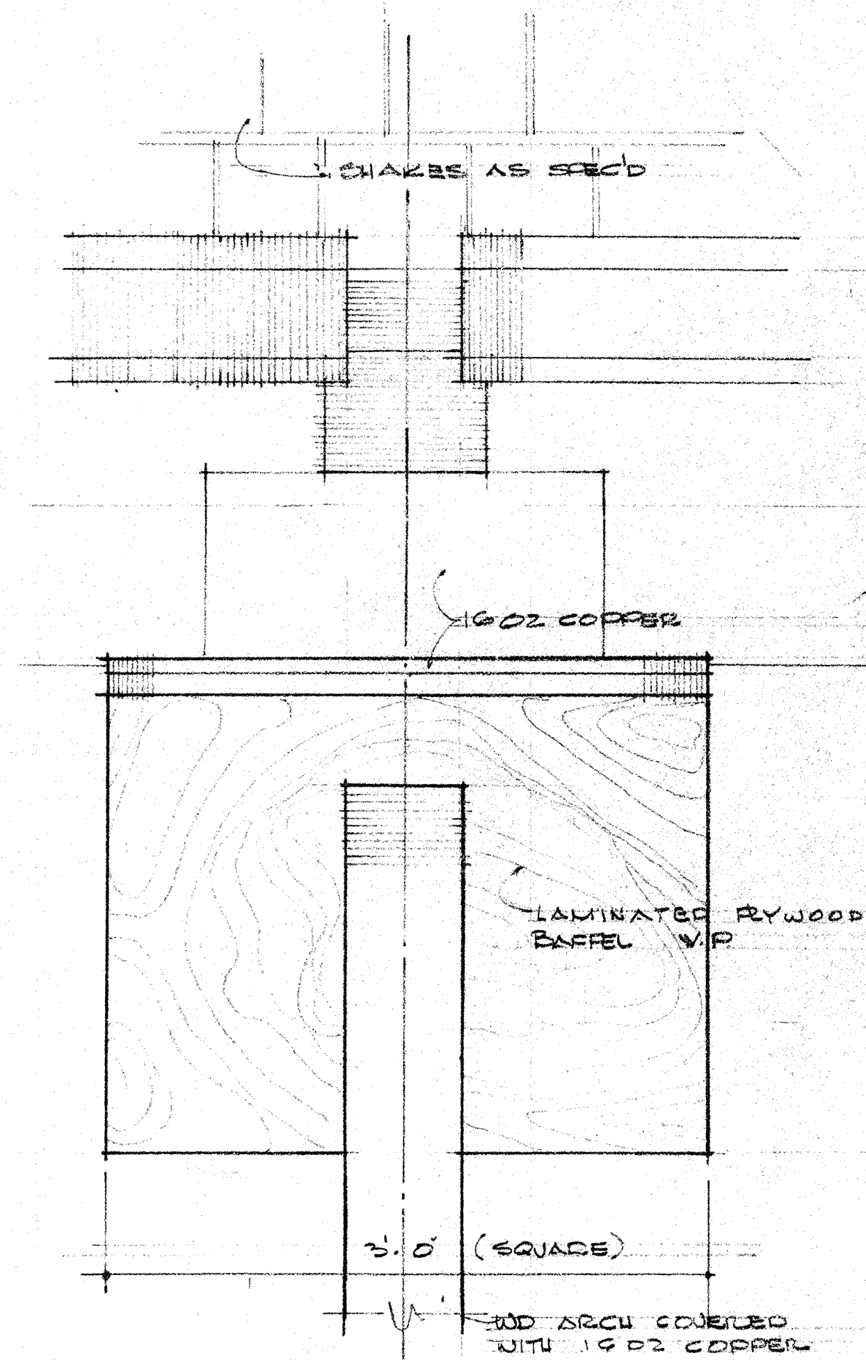
DETAIL \frac{D}{5} SCALE \frac{1}{2} = 1'-0"
