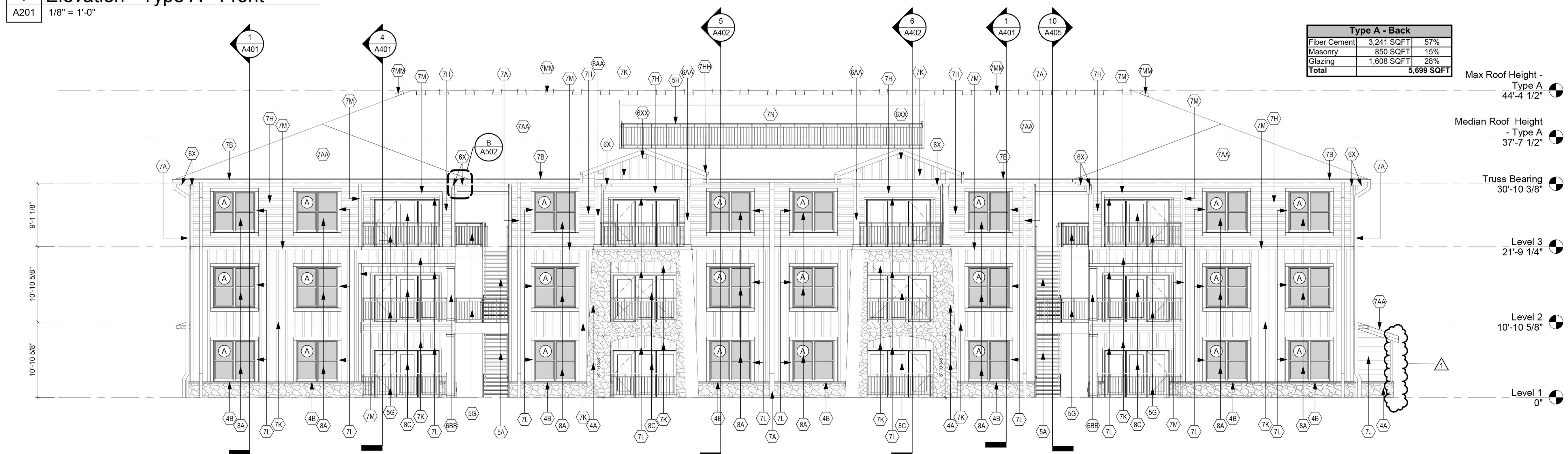
2 Elevation - Type A - Rear
