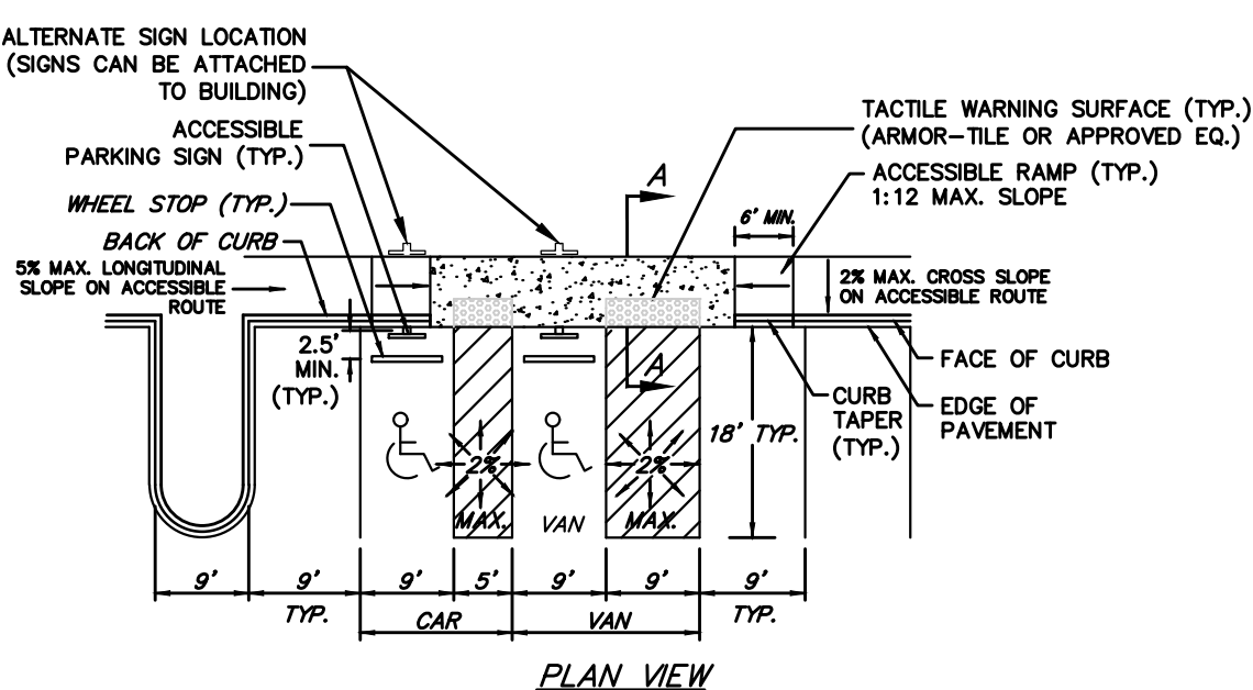
TYPICAL ACCESSIBLE PARKING SPACES NO SCALE
