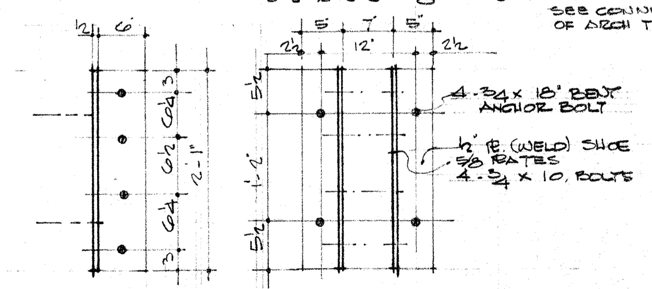
ELEV. BASE CONNECTION (SIDE) and PLAN OF BASE CONNECTION SCALE 1" = 1'-0"
