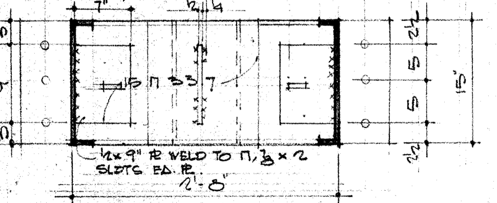
SECTION THRU COMPRESSION RING SCALE 1" = 1'-0"
