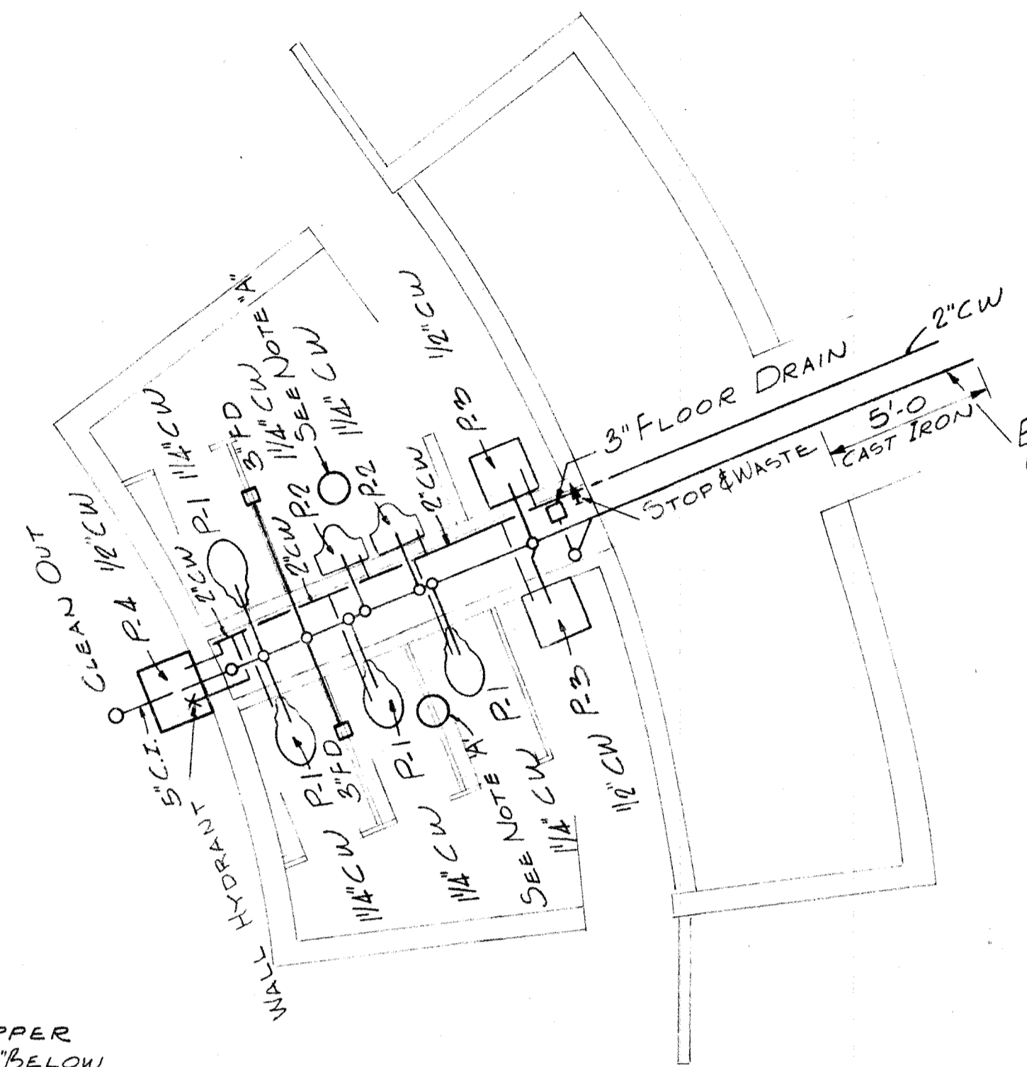
PART FLOOR PLAN SCALE 1/4"=1'-0"
