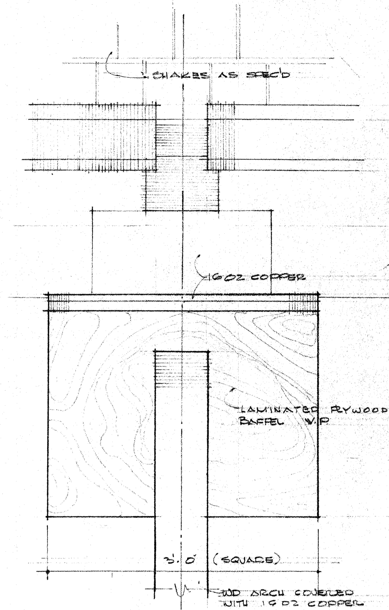
DETAIL D / 5 SCALE 1/2" = 1'-0"
