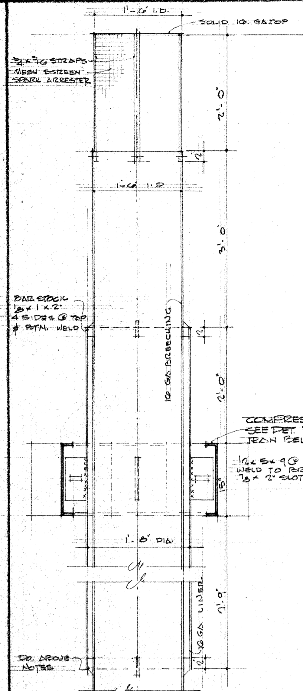
PART SECTION OF STACK SCALE 1" = 1'-0"
