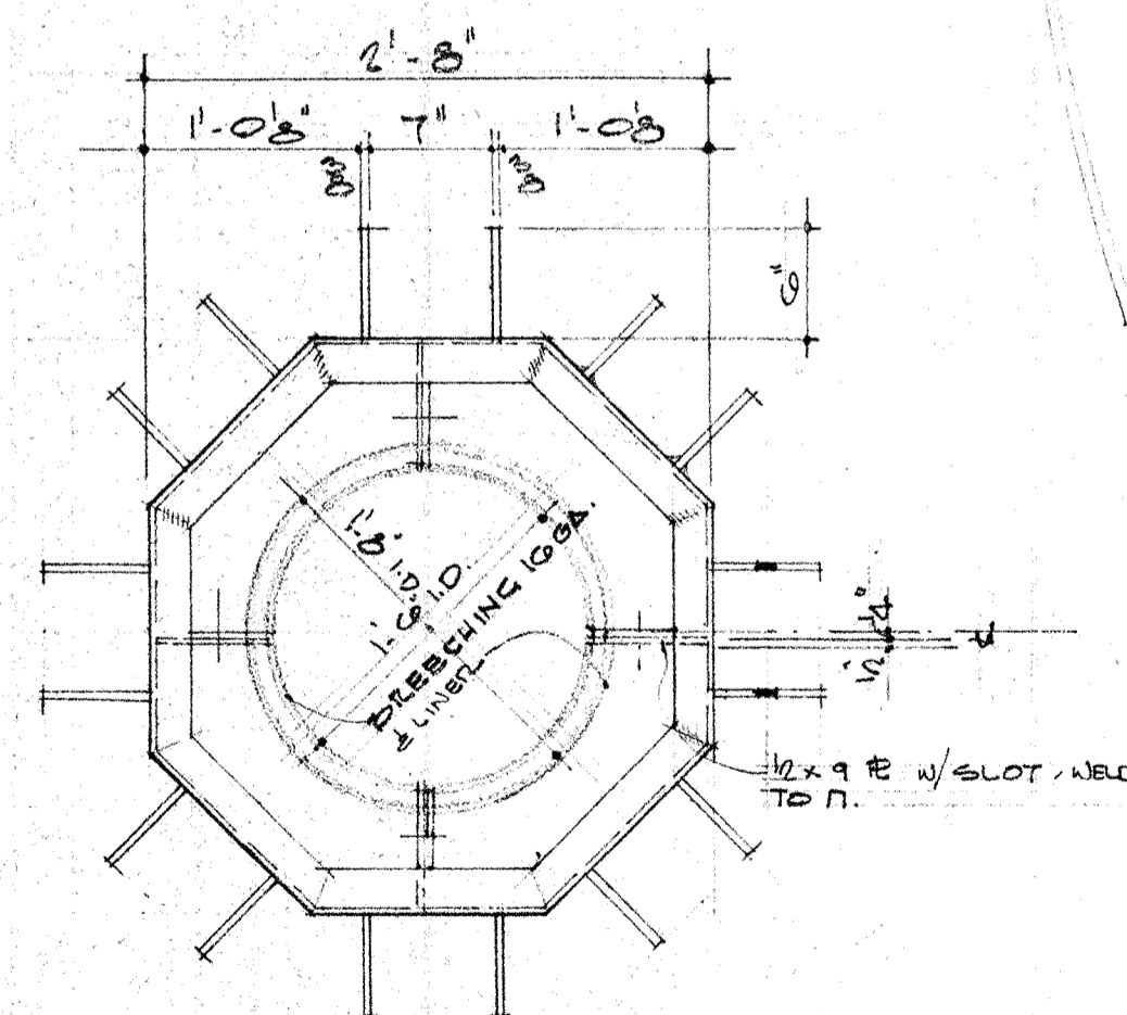
PLAN OF COMPRESSION RING SCALE 1" = 1'-0"
