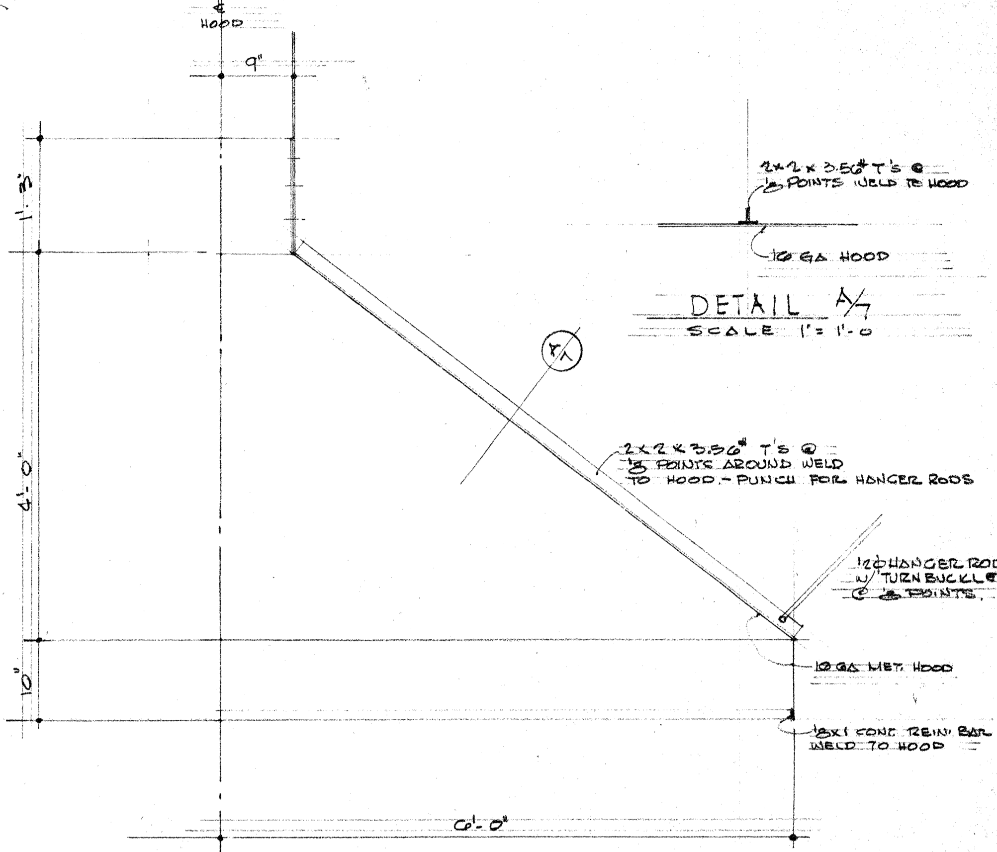
HALF SECTION THRU FIREPLACE HOOD SCALE 1" = 1'-0"
