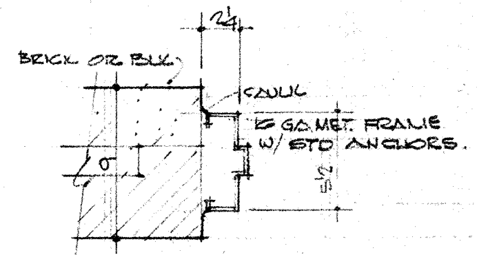
DETAIL TYP. DOOR JAMB SCALE 1/2" = 1'-0" FLOOR PLAN SCALE 1/4" = 1'-0"
