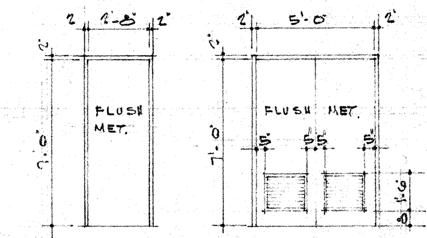
NO. 100 & 101 NO. 102 DOOR & FRAME TYPES SCALE 1/4" = 1'-0"
