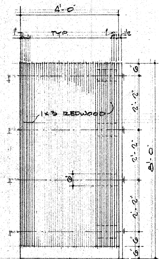
ELEVATION SCREEN WALL SCALE 1/2" = 1'-0"
