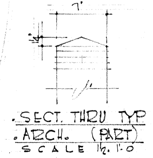
SECTION THRU TYP. ARCH. (PART) SCALE 1/2" = 1'-0"
