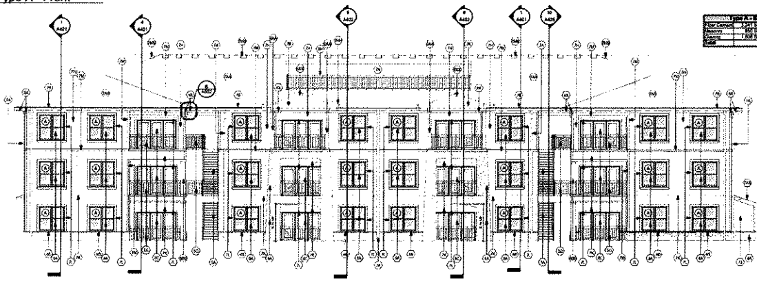
2 Elevation - Type A - Rear A201 1/8" = 1'-0"
