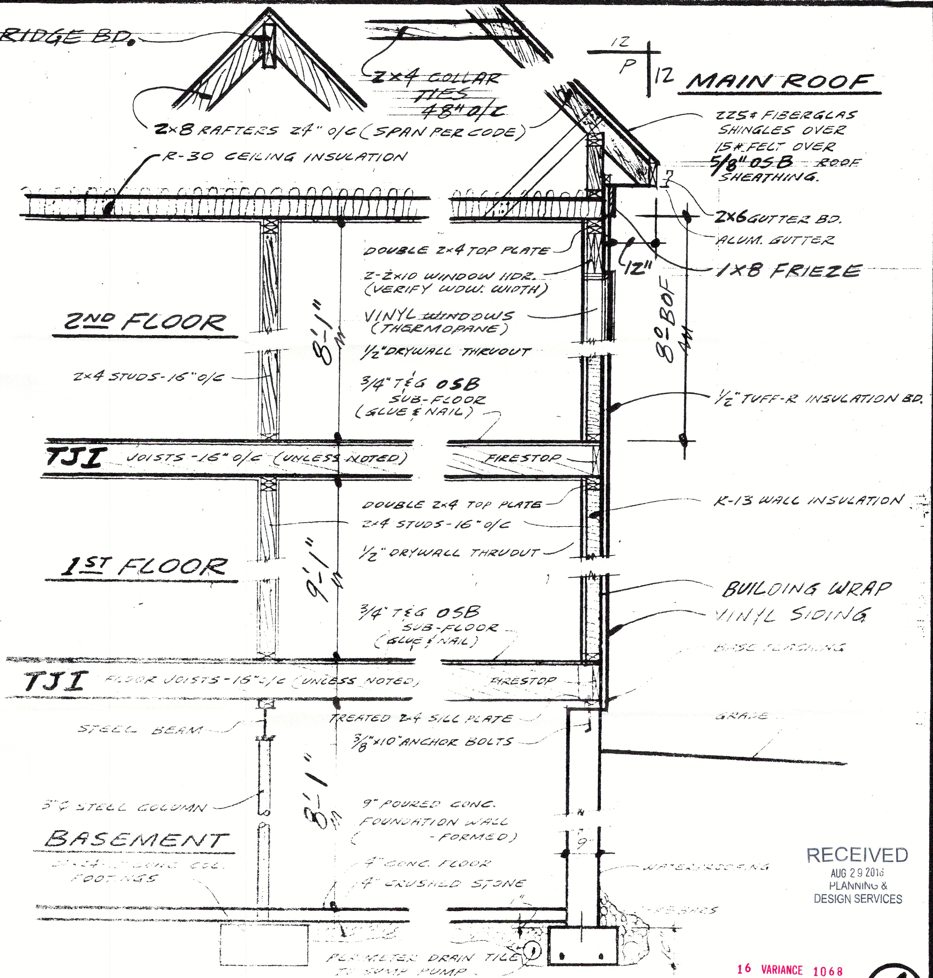
TYPICAL WALL SECTION 3/4" = 1'-0"
