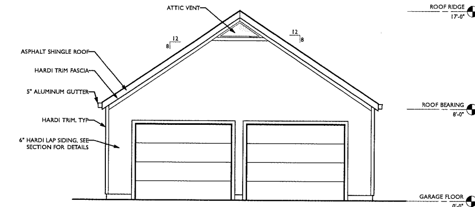
5 EAST ELEVATION Scale: 1/4" = 1'-0"
