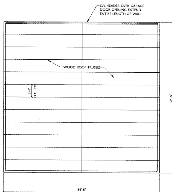
3 GARAGE FRAMING PLAN Scale: 1/4" = 1'-0"
