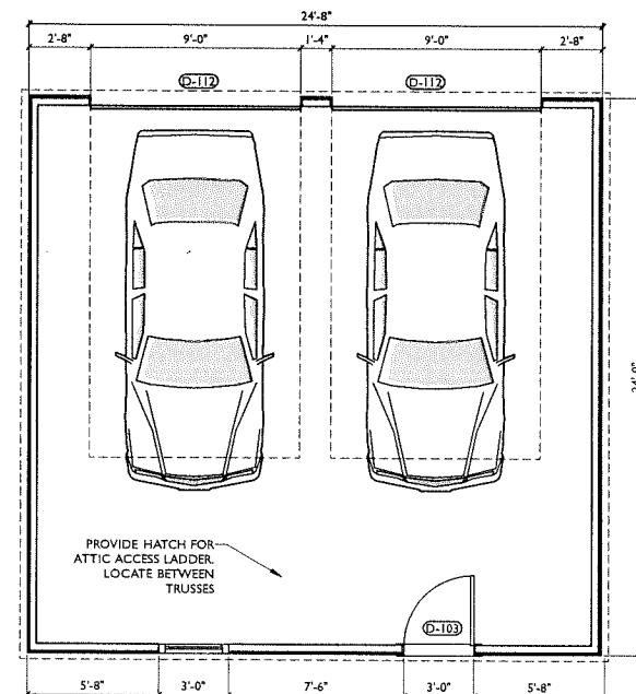
1 GARAGE FLOOR PLAN Scale: 1/4" = 1'-0"
