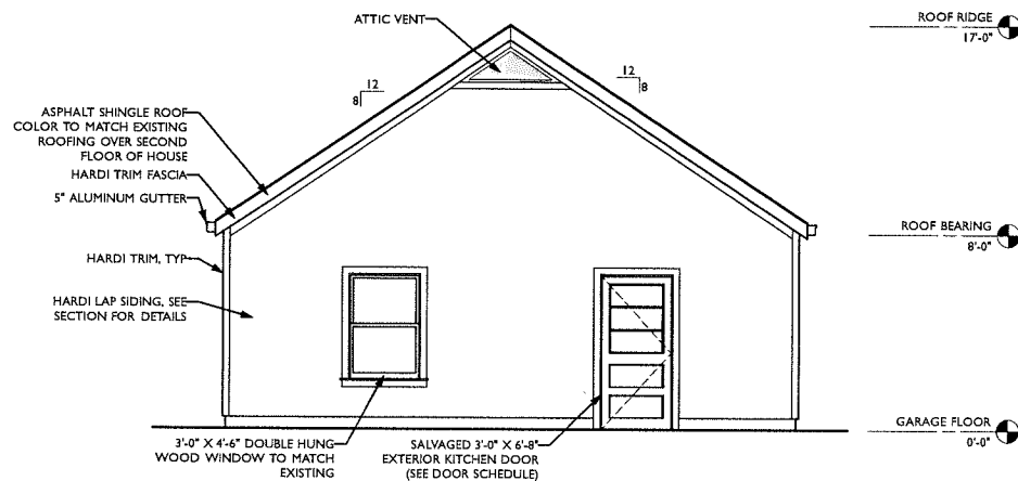
4 WEST ELEVATION Scale: 1/4" = 1'-0"
