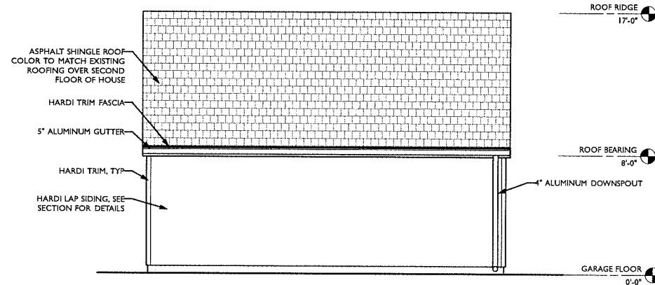
6 SIDE ELEVATIONS Scale: 1/4" = 1'-0"
