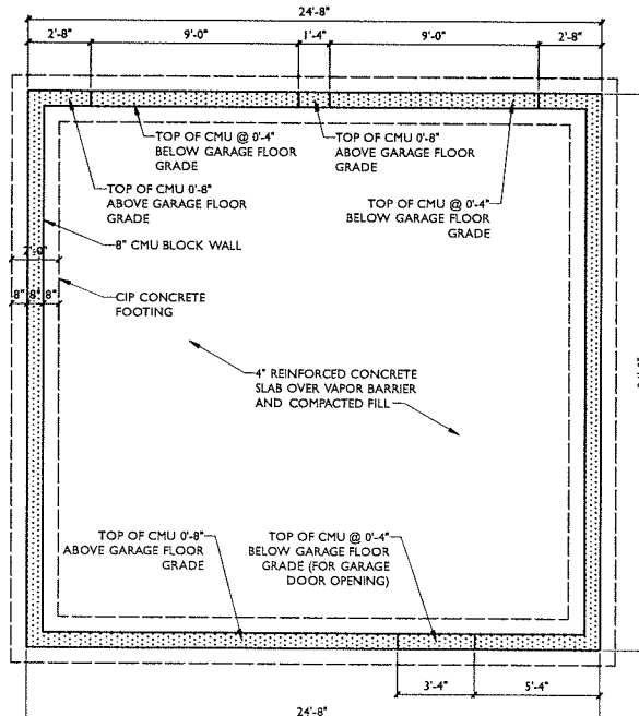
2 GARAGE FOUNDATION PLAN Scale: 1/4" = 1'-0"
