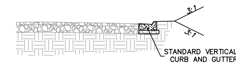
TYPICAL 2' CURB SECTION NO SCALE
