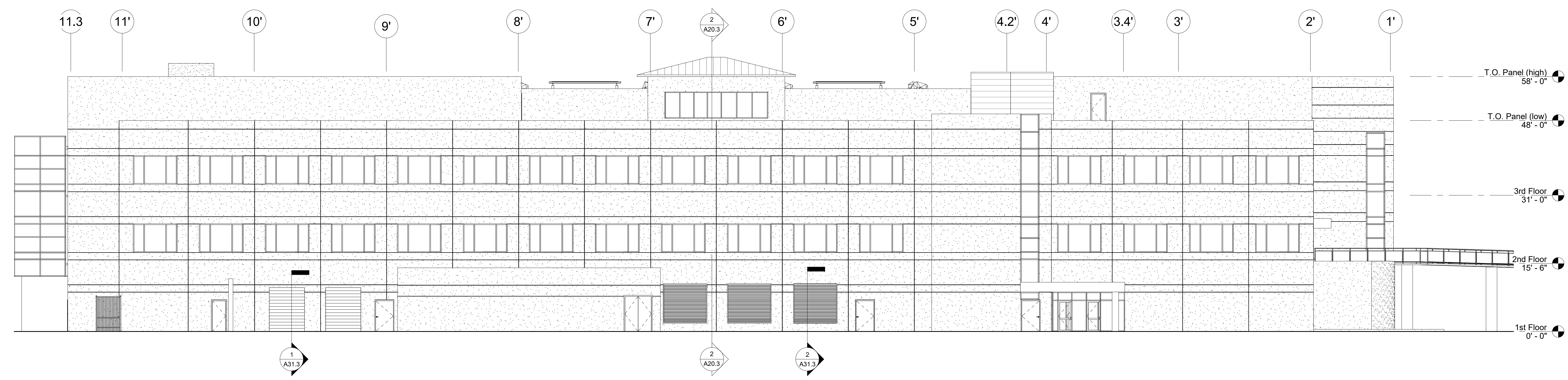
1 East Elevation 3/32" = 1'-0"
