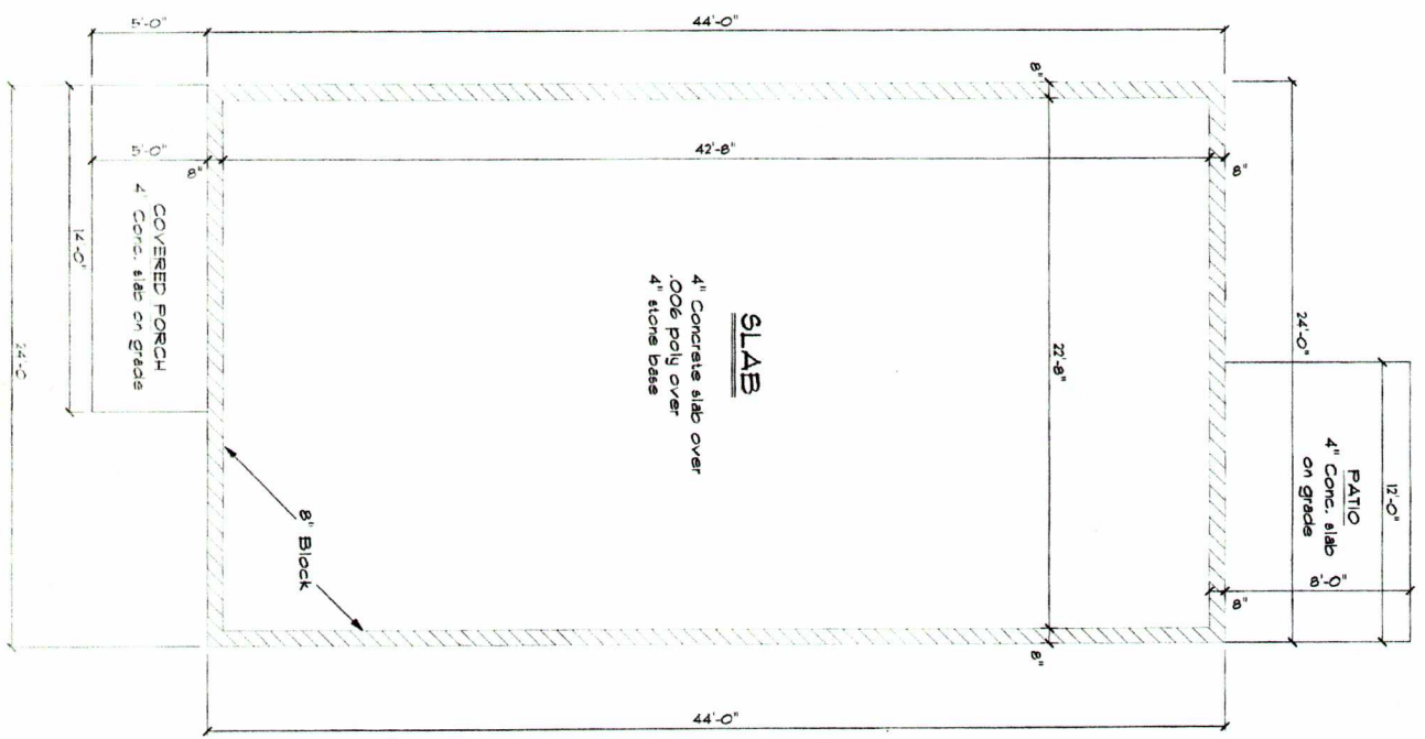
FOUNDATION PLAN
