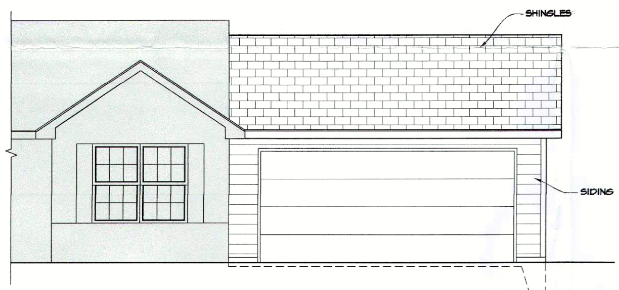
FRONT ELEVATION 1/4"=1'-0"
