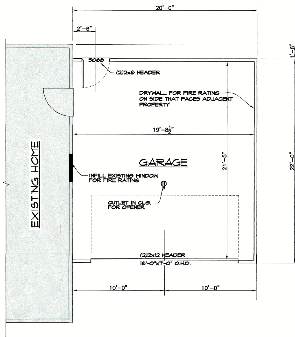
GARAGE FLOOR PLAN 1/4"=1'-0"
