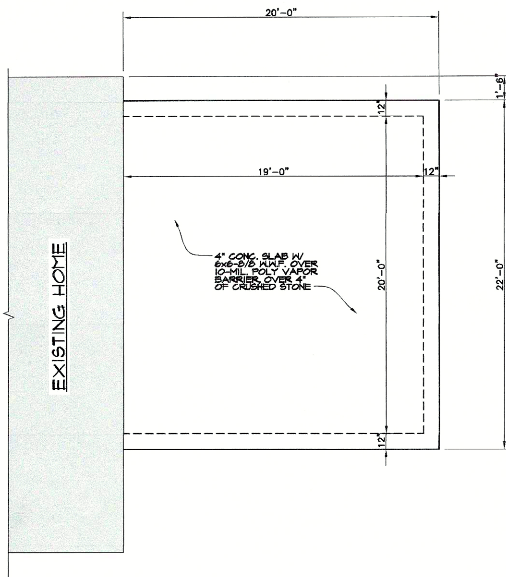
FOUNDATION PLAN 1/4"=1'-0"
