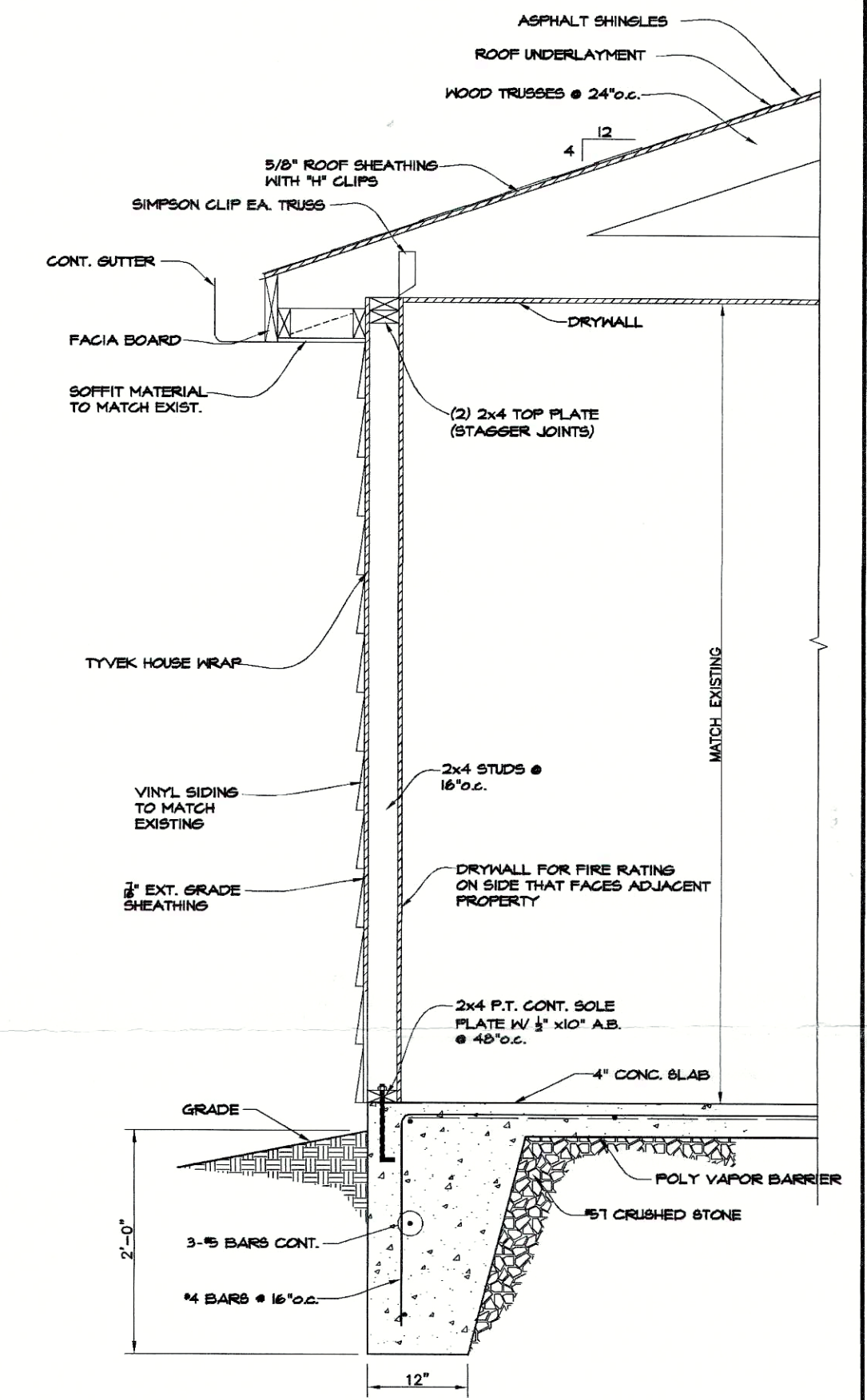
TYPICAL FOUNDATION SECTION W/VINYL
