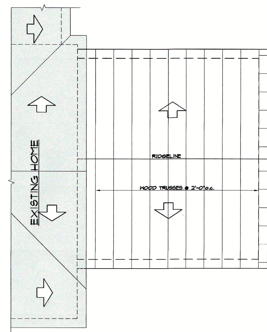
ROOF PLAN 1/4"=1'-0"
