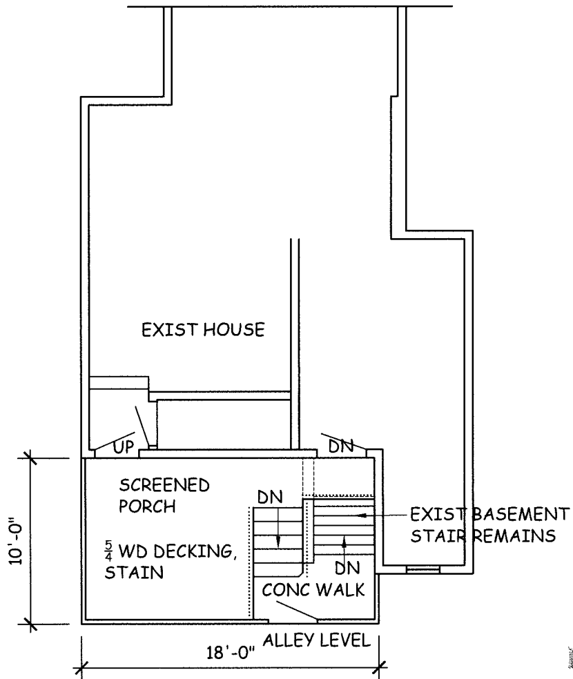
SCREENED PORCH PLAN
