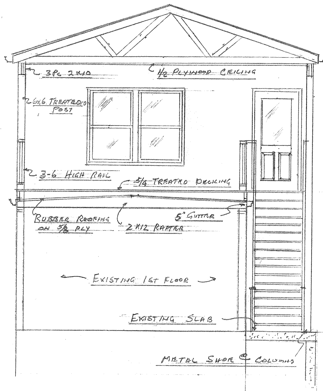
SOUTH ELEVATION @ DECK.
