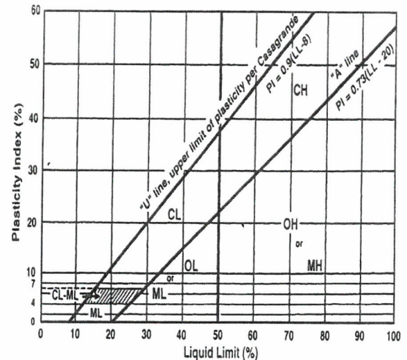
Plasticity Chart
