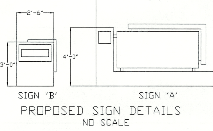
PROPOSED SIGN DETAILS NO SCALE
