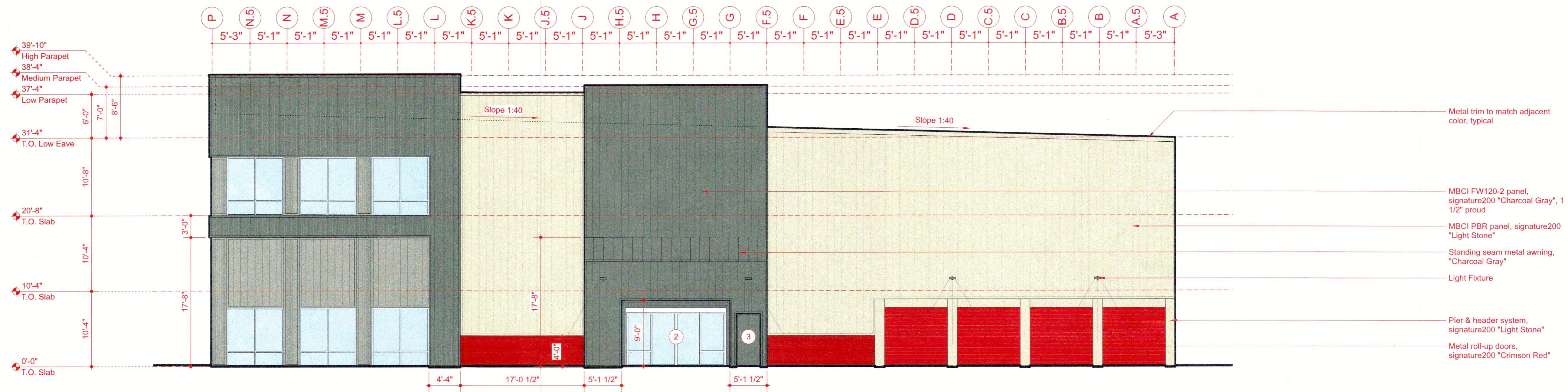
SOUTH ELEVATION A2.18 1/8"
