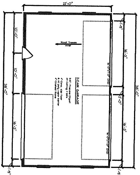
FLOOR PLAN 1/4" = 1'-0" TTC
