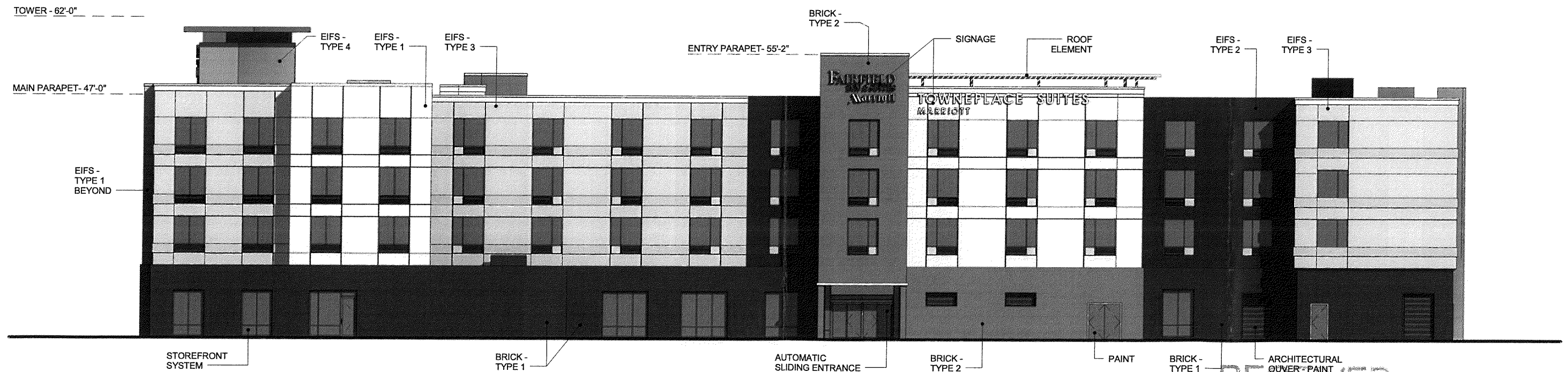
NORTH ELEVATION
