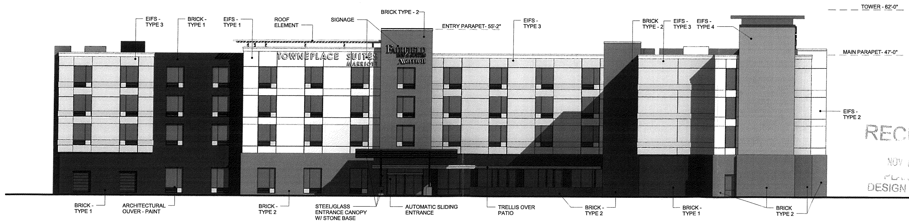
SOUTH ELEVATION
