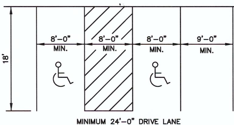
TYPICAL PARKING SPACE LAYOUT
