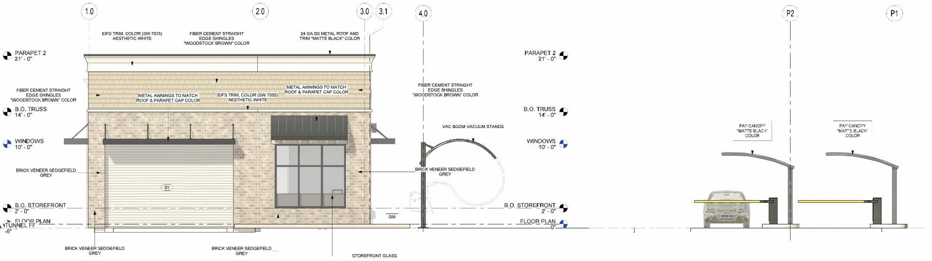
1 NORTH REAR ELEVATION A105 : 1/4" = 1'-0"
