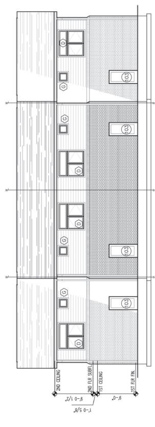
BUILDING TYPE - "C" REAR ELEVATION
