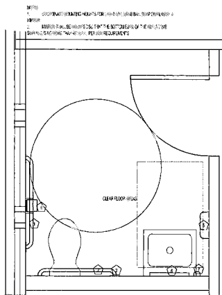
ENLARGED TOILET PLAN SCALE: 3/4" = 1'-0"
