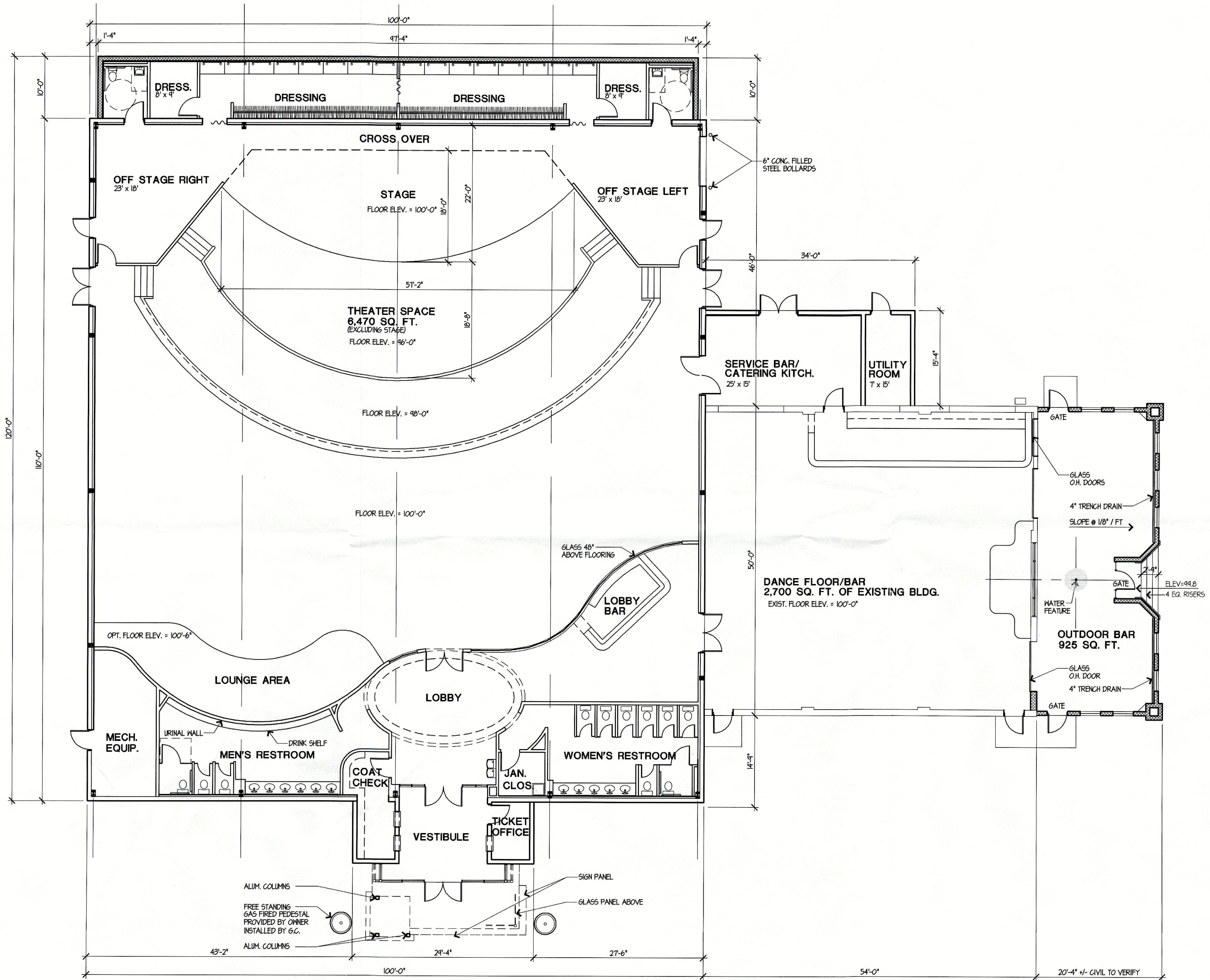
SCHEMATIC FLOOR PLAN H SCALE = 3/32" = 1'-0"
