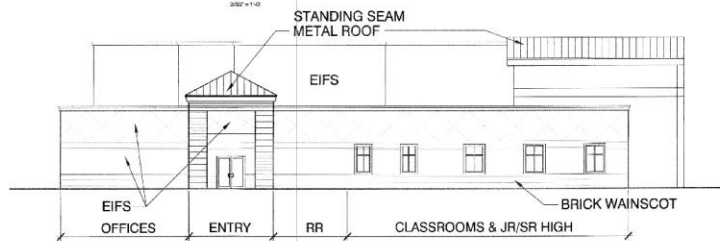
PRELIMINARY ELEVATION
