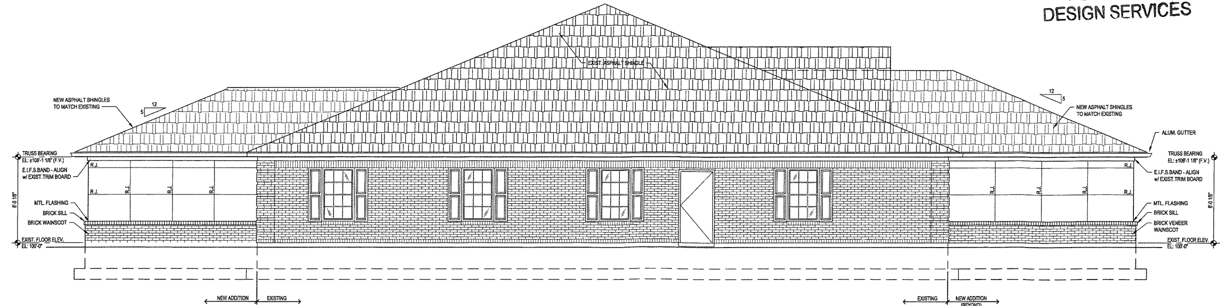
2 WEST (LEFT SIDE) ELEVATION A2.1 SCALE: 1/4" = 1'-0"
