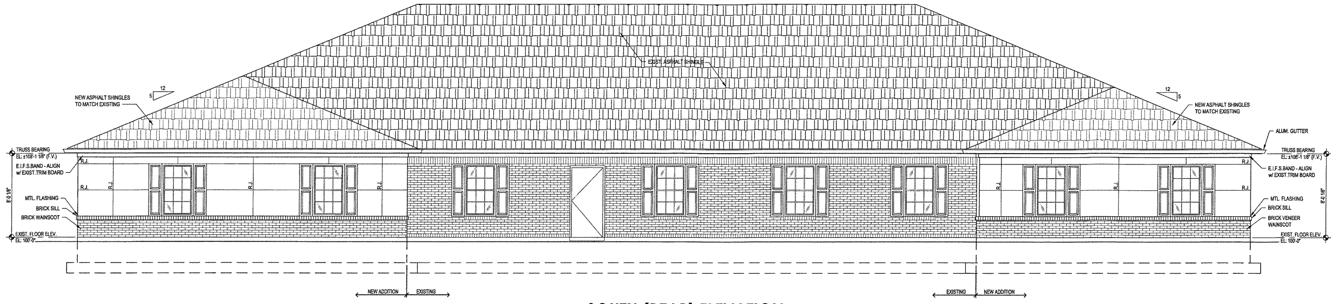
1 SOUTH (REAR) ELEVATION A2.1 SCALE: 1/4" = 1'-0"
