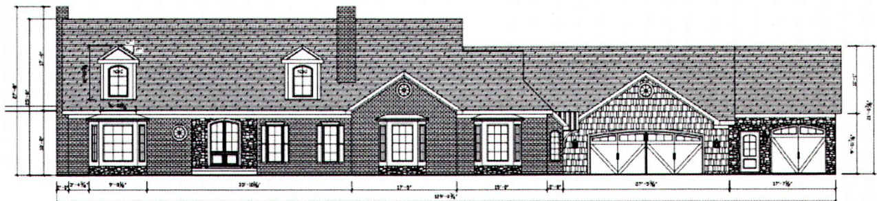
FRONT ELEVATION
