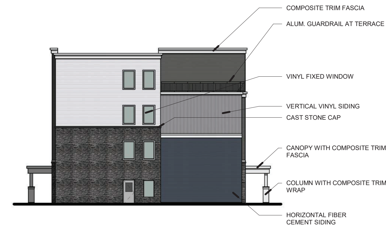
3 PR4.2 BUILDING B - WEST ELEVATION 1/16" = 1'-0"
