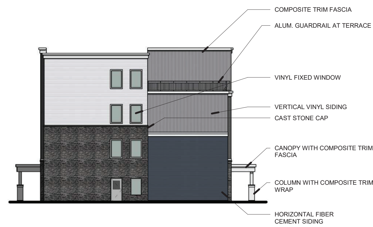
3 BUILDING A - SOUTH ELEVATION PR4.1 1/16" = 1'-0"
