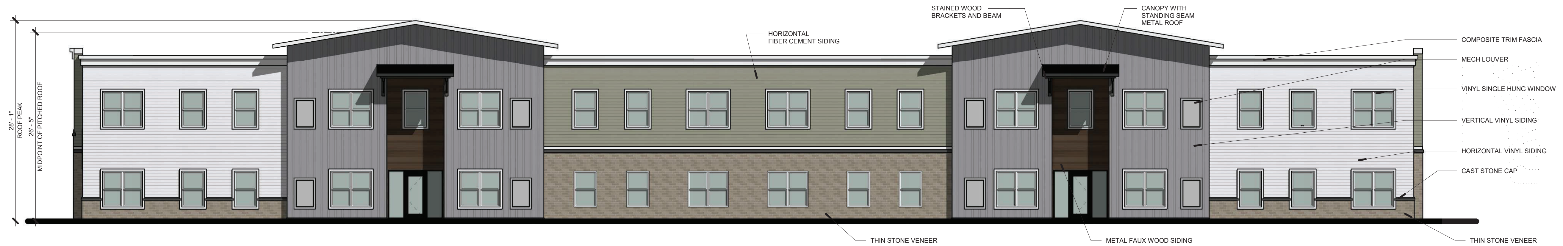
3 BLDG E - FRONT ELEVATION (REAR SIM.) PR4.4 1/8" = 1'-0"
