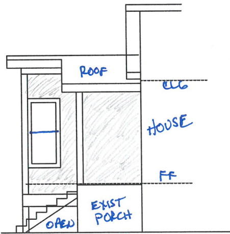
STREET SIDE ELEVATION
