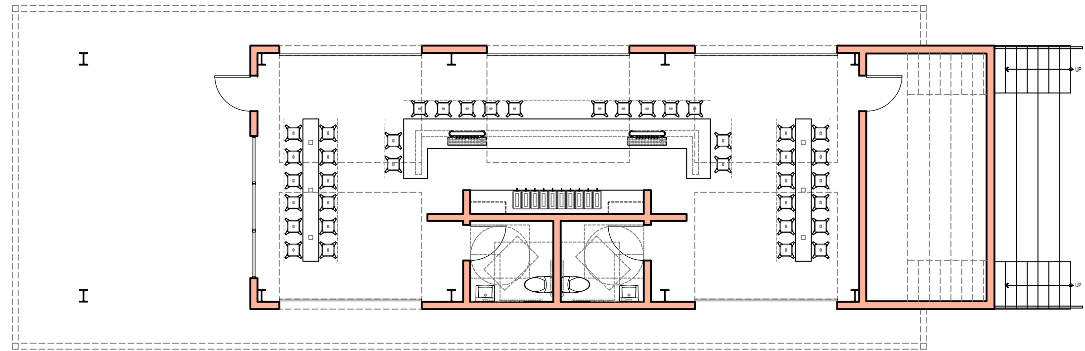
2 PAVILION - First Floor Plan S.1 scale: 1/8" = 1'-0"
