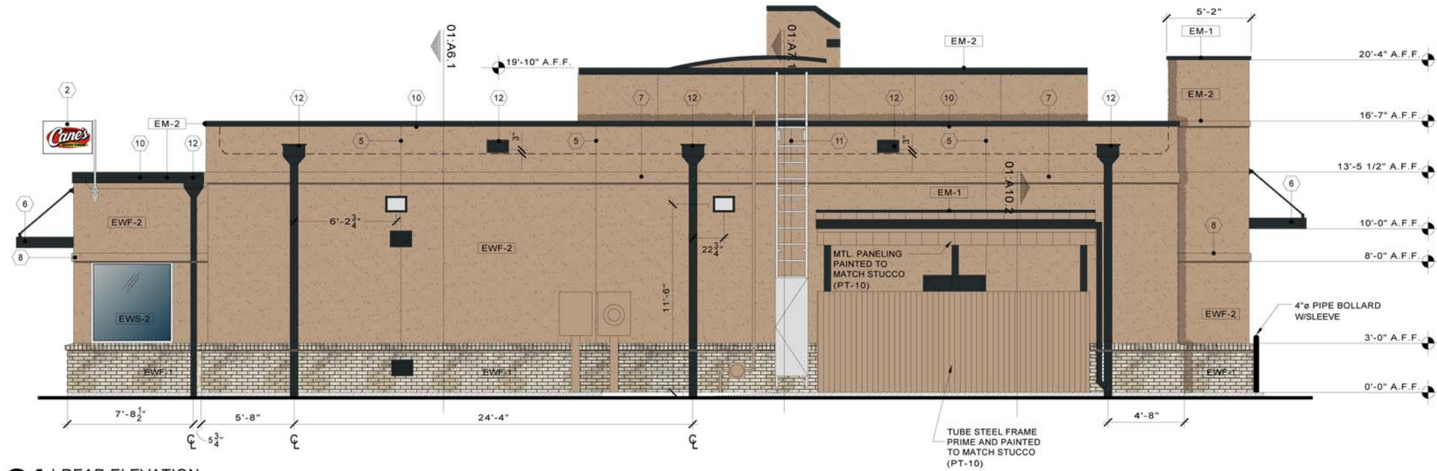
01 REAR ELEVATION 1/4" = 1'-0" 01:A4.2
