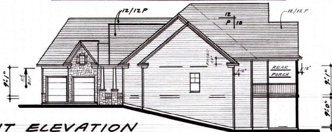
LEFT ELEVATION
