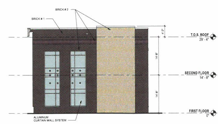
4 PARTIAL WEST ELEVATION 'A' SCALE: 1/8" = 1'-0"
