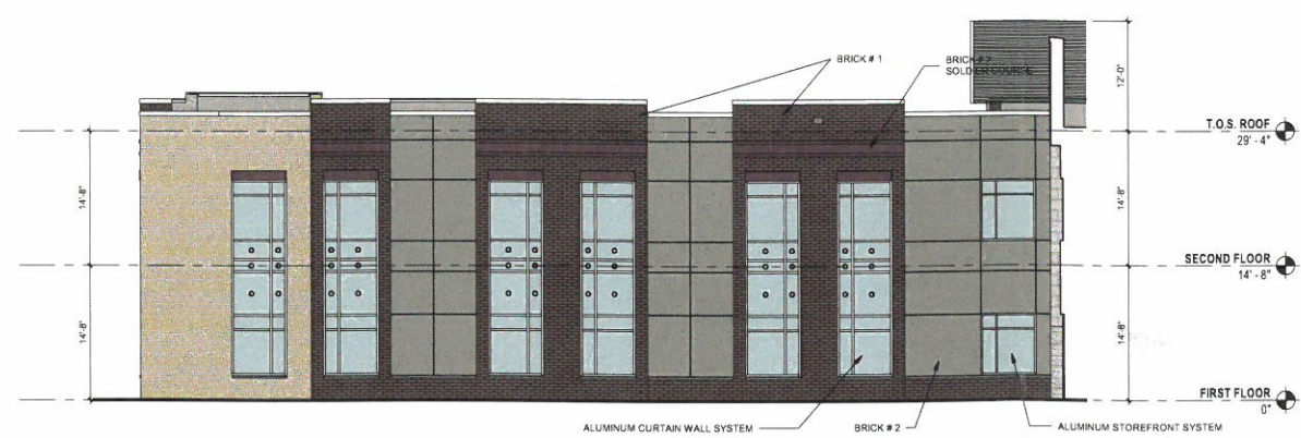
3 PARTIAL EAST ELEVATION SCALE: 1/8" = 1'-0"
