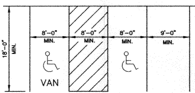
TYPICAL PARKING SPACE LAYOUT NO SCALE
