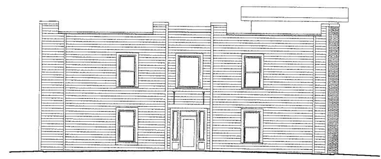
4 BUILDINGS 5,12 - REAR ELEVATION 1/8" = 1'-0"
