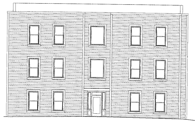
4 BUILDING 14 - REAR ELEVATION 1/8" = 1'-0"
