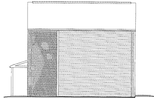
3 BUILDINGS 7,9 - RIGHT SIDE ELEVATION 1/8" = 1'-0"
