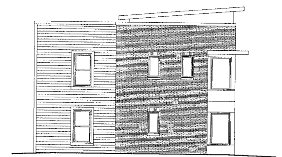
2 BUILDINGS 5,12 - LEFT SIDE ELEVATION 1/8" = 1'-0"
