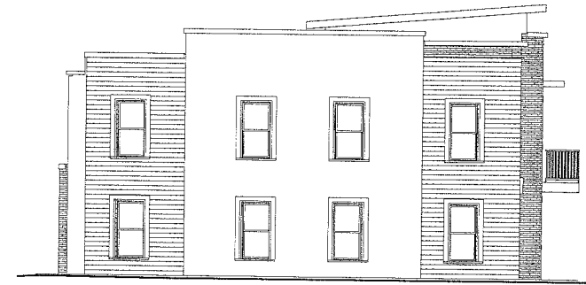
2 BUILDING 11 - LEFT SIDE ELEVATION 1/8" = 1'-0"
