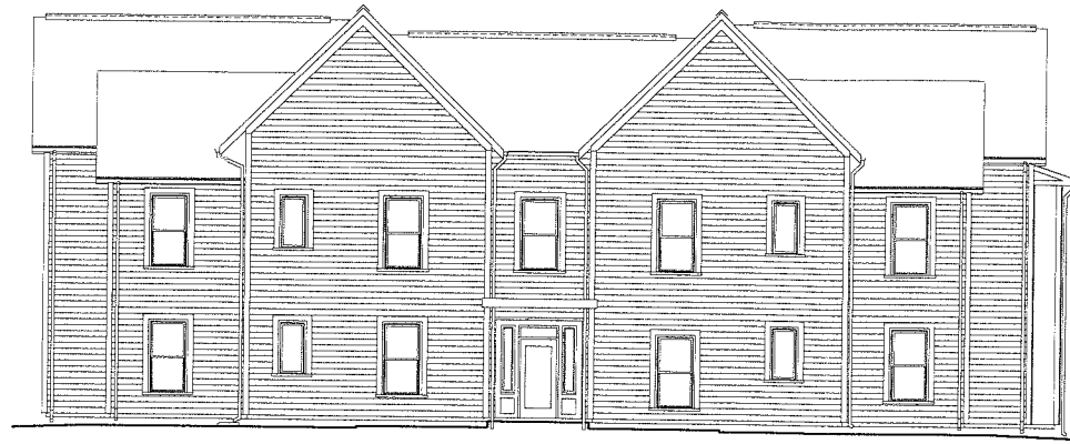
4 BUILDING 1 - REAR ELEVATION 1/8" = 1'-0"
