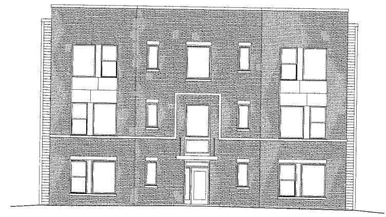
1 BUILDING 14 - FRONT ELEVATION 1/8" = 1'-0"
