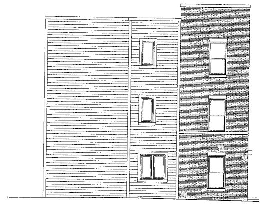
2 BUILDING 14 - LEFT ELEVATION 1/8" = 1'-0"
