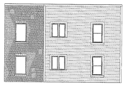
3 BUILDINGS 5,12 - RIGHT SIDE ELEVATION 1/8" = 1'-0"
