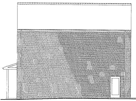
3 BUILDINGS 6,8,10 - RIGHT SIDE ELEVATION 1/8" = 1'-0"
