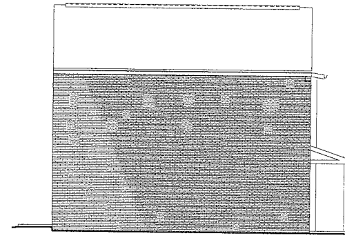
2 BUILDINGS 7,9 - LEFT SIDE ELEVATION 1/8" = 1'-0"
