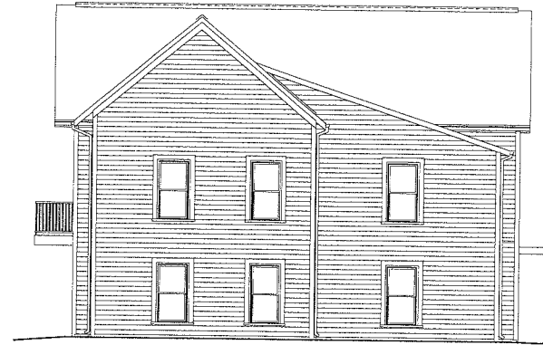
3 BUILDING 1 - RIGHT SIDE ELEVATION 1/8" = 1'-0"
