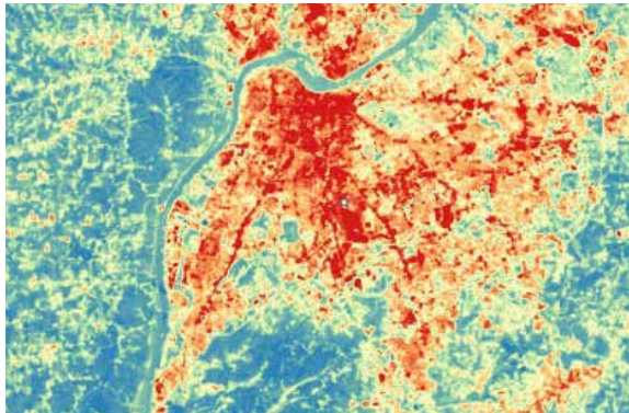
Urban heat measured by satellite in Louisville. Image Source: Climate Central
