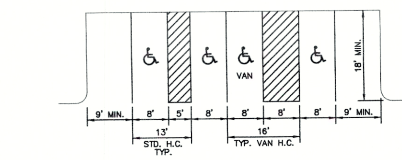
TYPICAL PARKING SPACES NO SCALE
