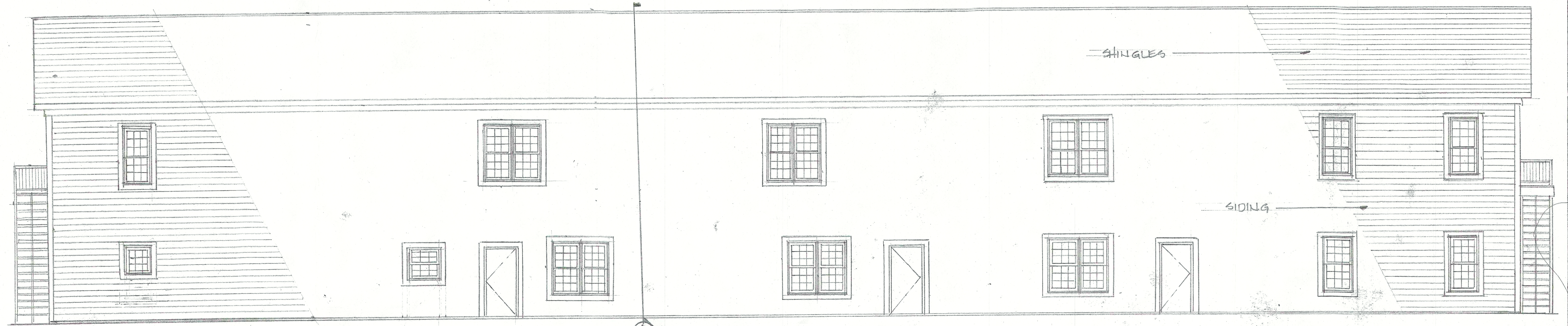
REAR ELEVATION
