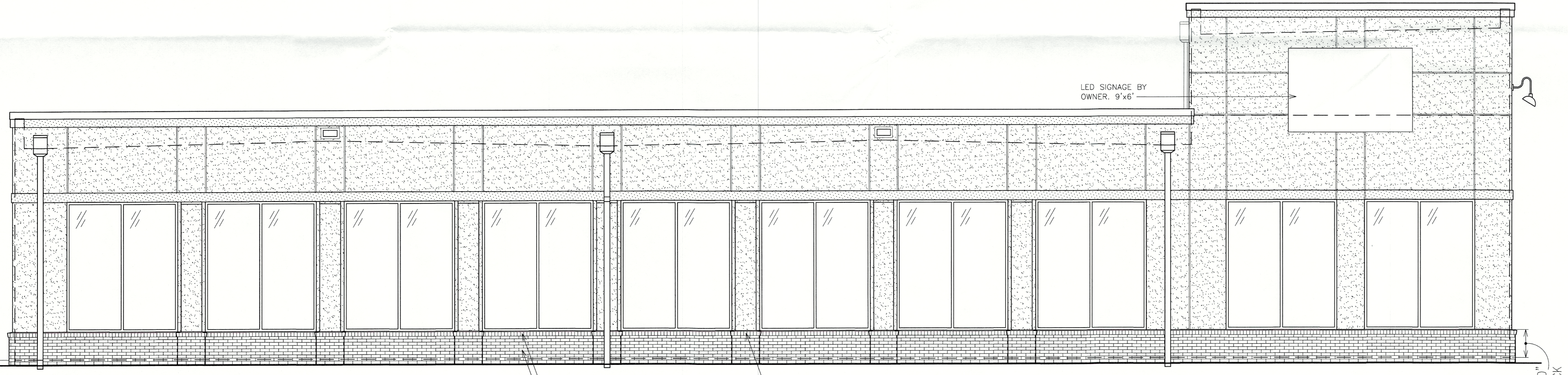
A1 TUNNEL ELEVATION 1/4" = 1'-0"
