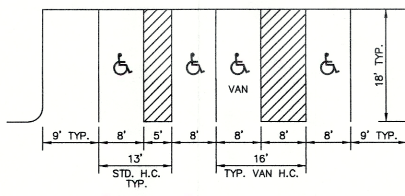
TYPICAL PARKING SPACES NO SCALE
