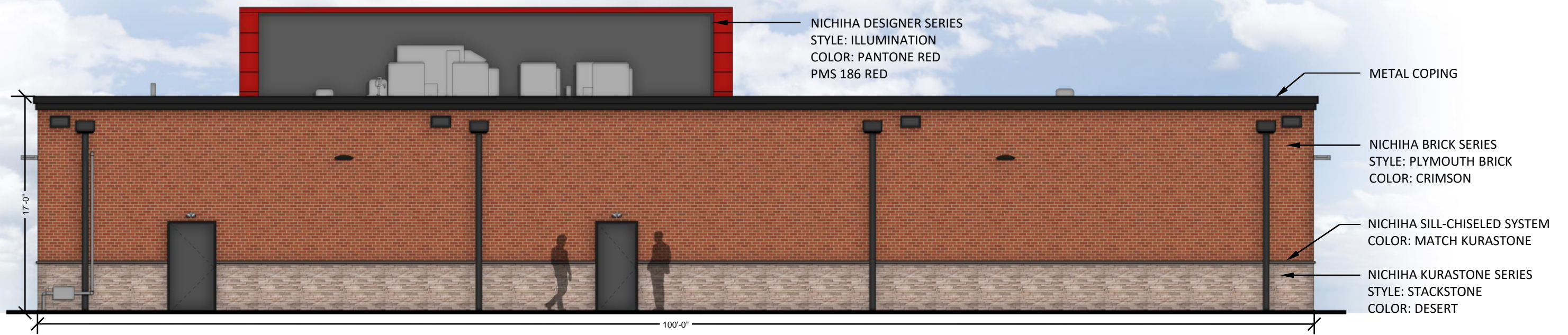
REAR ELEVATION
