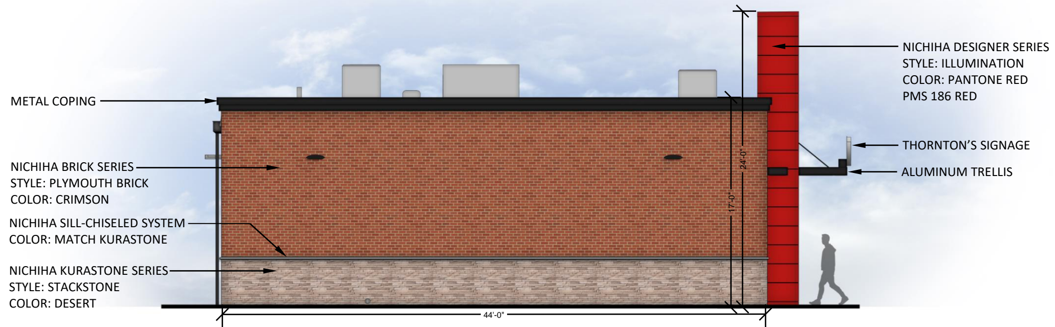
SIDE ELEVATION
