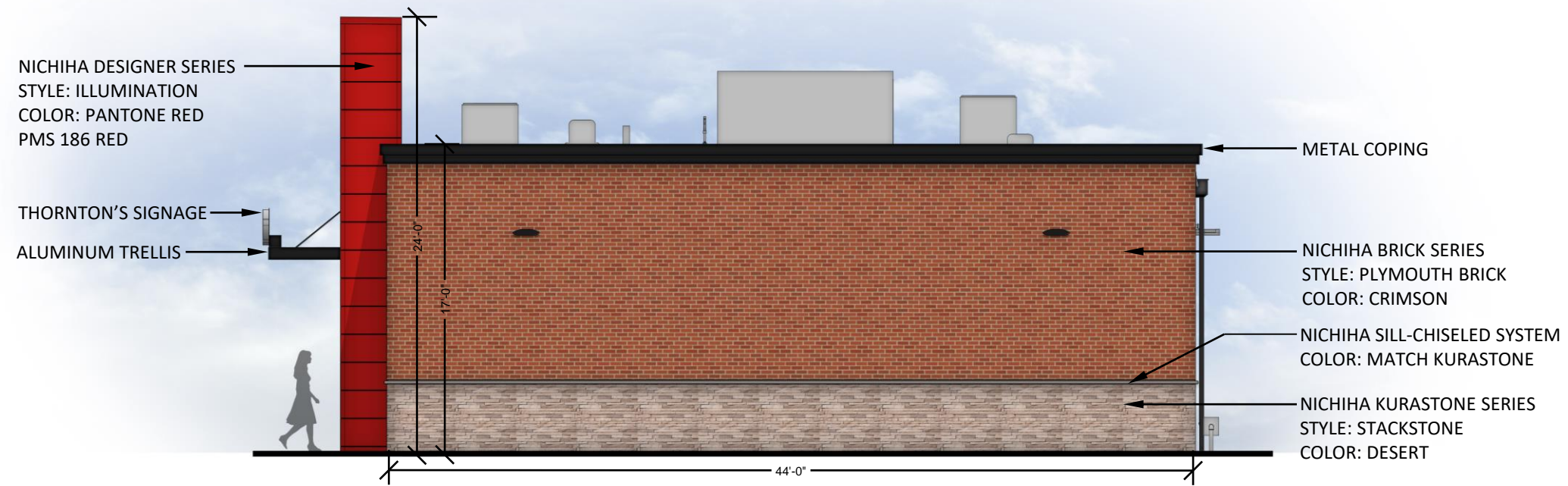
SIDE ELEVATION
