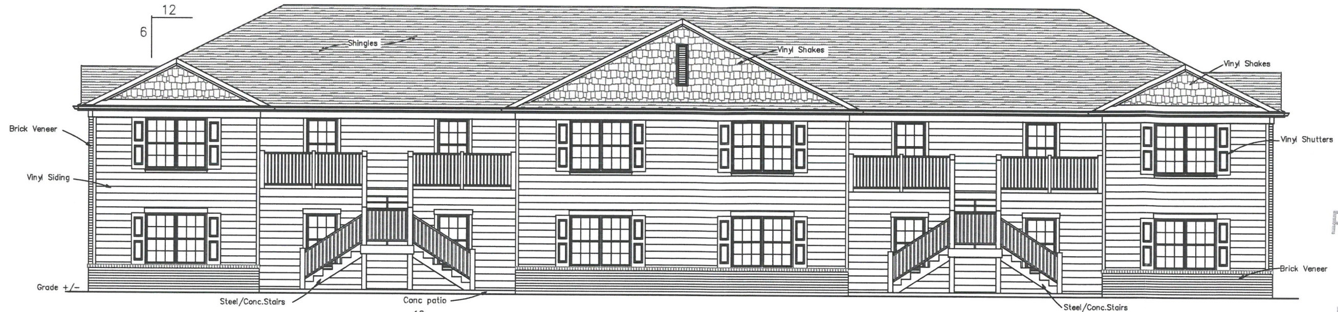
FRONT ELEVATION
