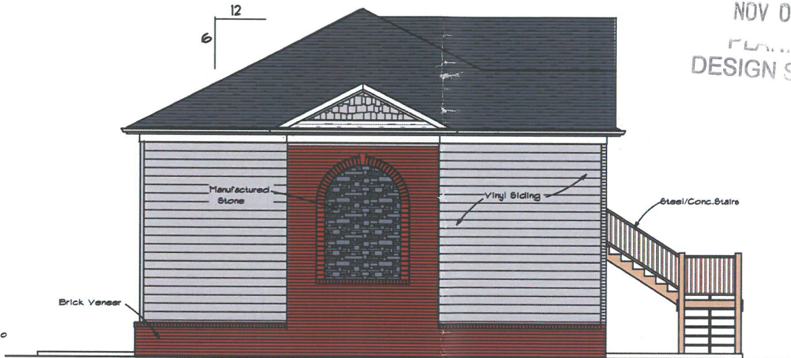
LEFT ELEVATION
