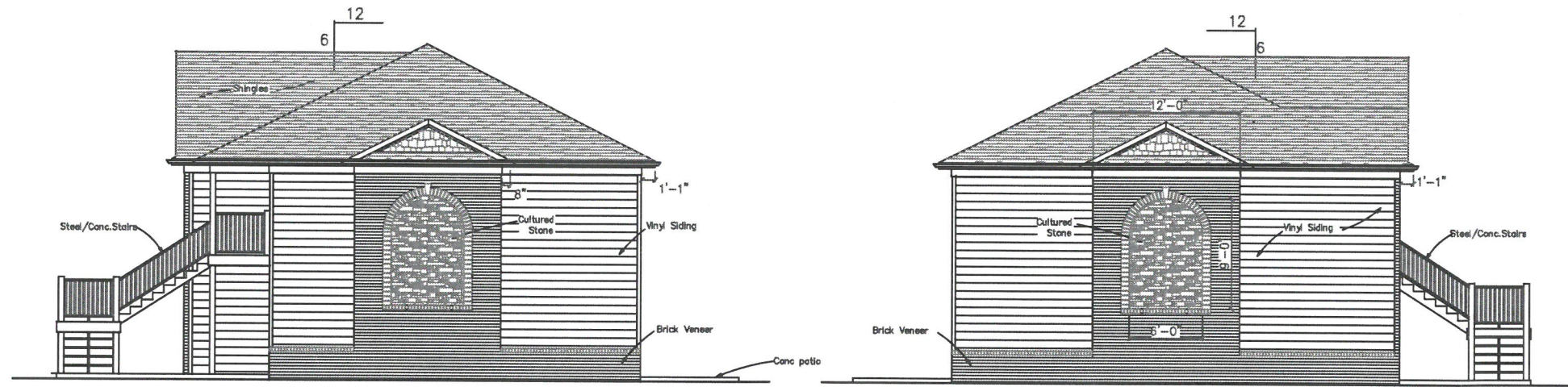
RIGHT ELEVATION 1/4"=1'-0"
