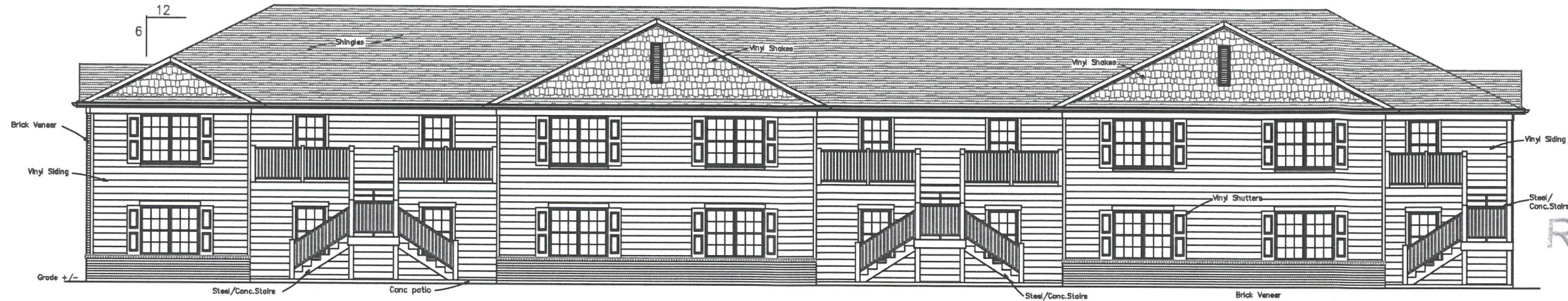
FRONT ELEVATION 1/4"=1'-0" 9,930 Total Sq Ft +/-
