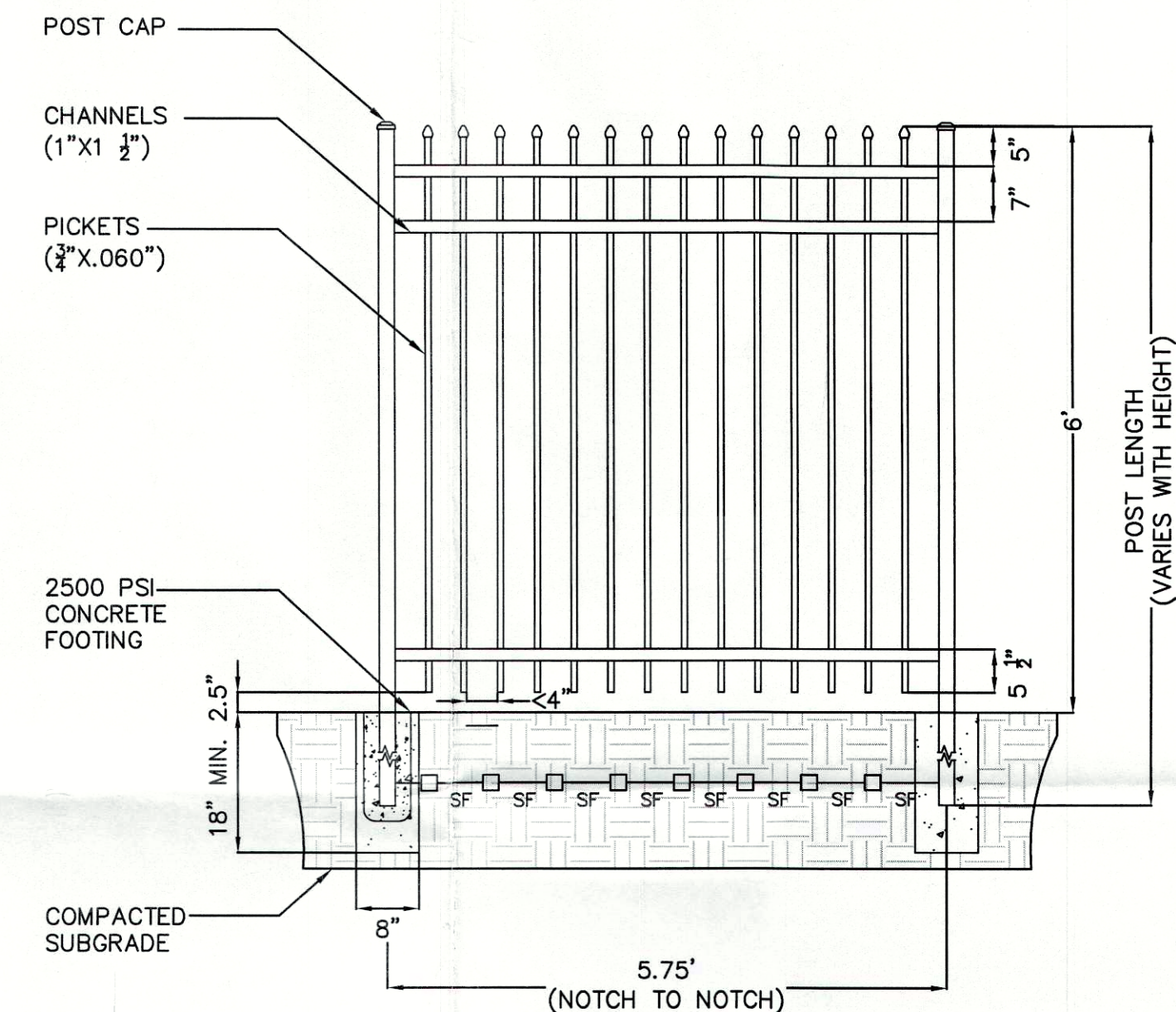
PERIMETER SECURITY FENCE (IDEAL MAINE #203 6' FENCE PANEL) NO SCALE
