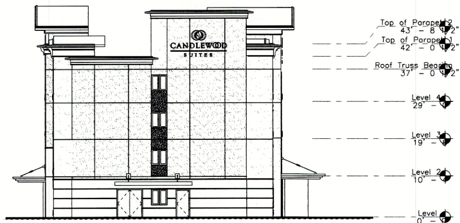
B LEFT ELEVATION 3/32" = 1'-0"
