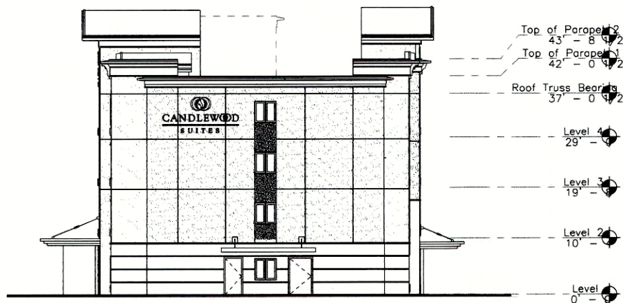
C RIGHT ELEVATION 3/32" = 1'-0"
