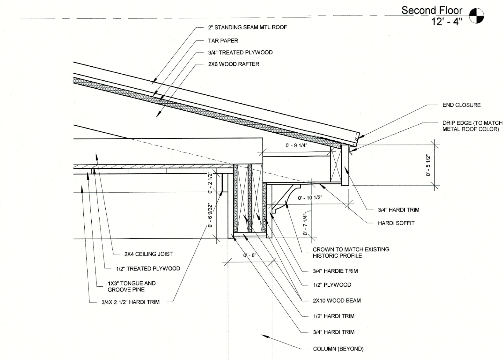
① DETAIL - FRONT PORCH 1 1/2" = 1'-0"
