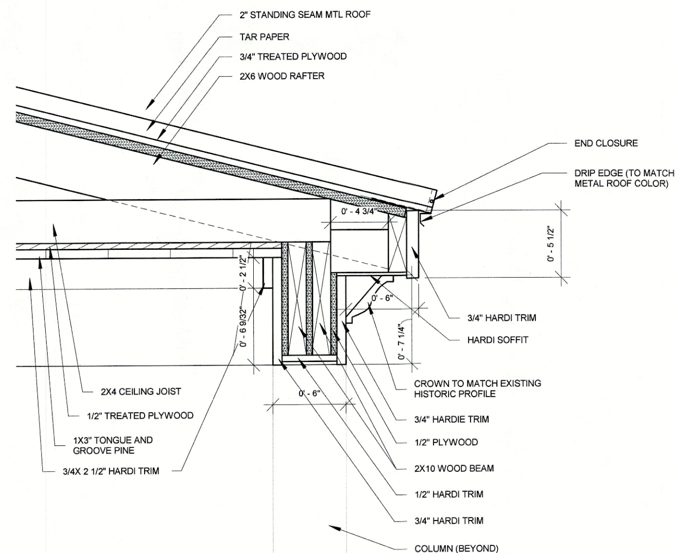
② DETAIL - SIDE PORCH 1 1/2" = 1'-0"
