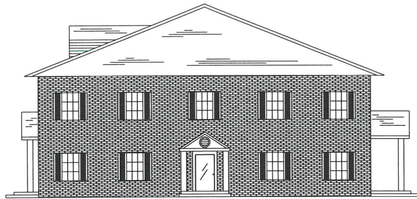
SIDE (ACCESS DRIVE)
