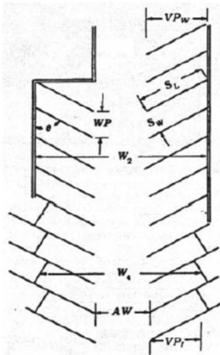
Figure 9.1.13 Parking Dimensional Layout Diagram
